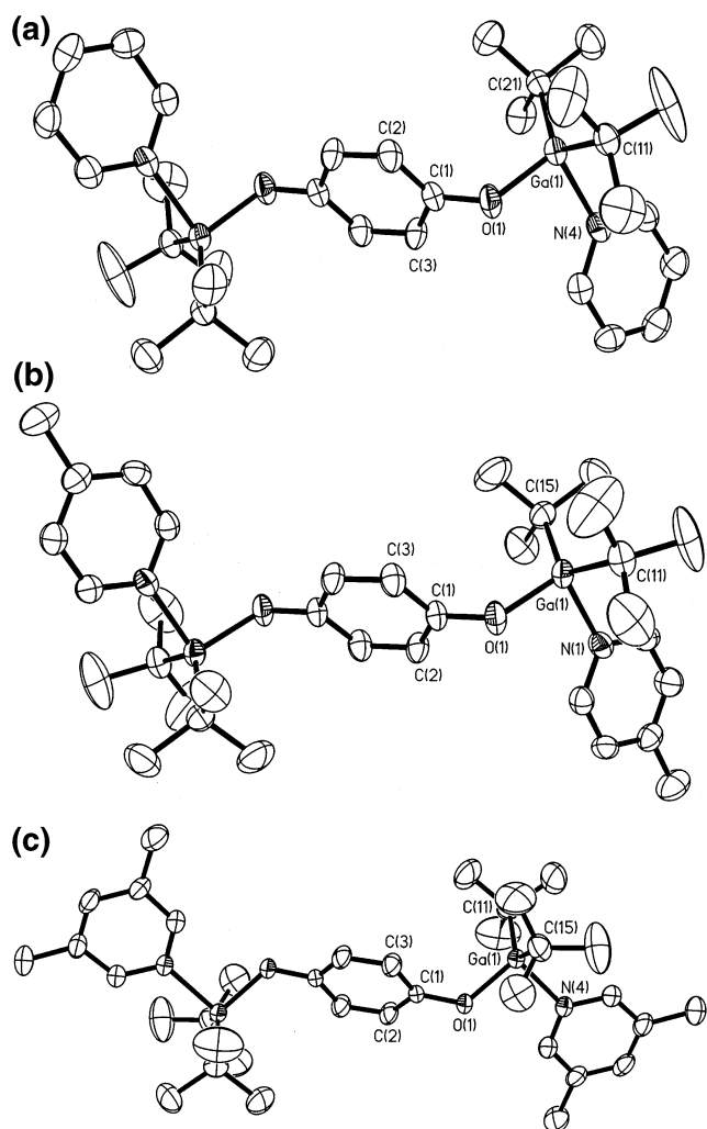
Figure 1. Molecular structures of (a) [(t\text{Bu})_2\text{Ga}(\text{py})]_2(\mu\text{-OC}_6\text{H}_4\text{O}) ( 2 ), (b) [(t\text{Bu})_2\text{Ga}(4\text{-Mepy})]_2(\mu\text{-OC}_6\text{H}_4\text{O}) ( 3 ) and (c) [(t\text{Bu})_2\text{Ga}(3,5\text{-Me}_2\text{py})]_2(\mu\text{-OC}_6\text{H}_4\text{O}) ( 4 ). Thermal ellipsoids shown at the 30% level, and hydrogen atoms are omitted for clarity.
