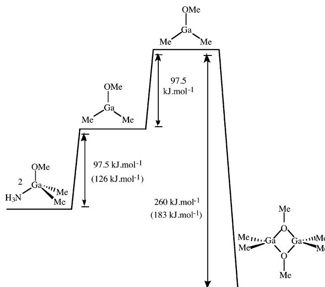
Figure 8. Calculated reaction diagram for the dissociative–dissociative pathway proposed to occur for the condensation/polymerization reaction of compounds 2 , 3 , and 5 in the solid state. Experimental values for compound 5 given in parentheses.
